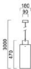
TOOL 26209.06 2x TC-L, 18W, 2G11
